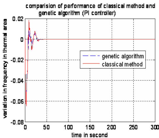
Figure 12. Frequency in thermal area v/s time
