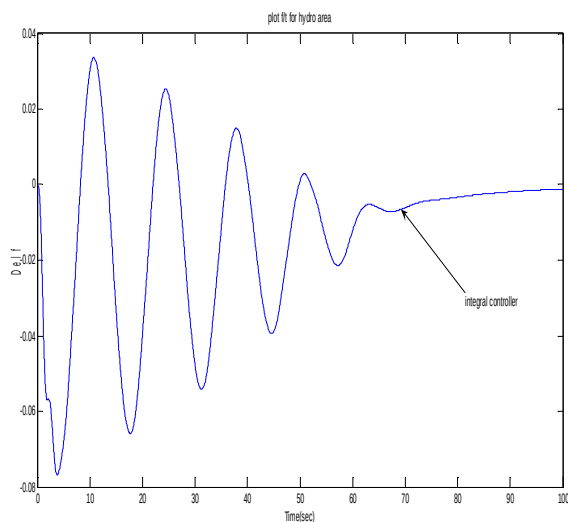
Figure 7. Variation of frequency for 1% step load change in hydro area
