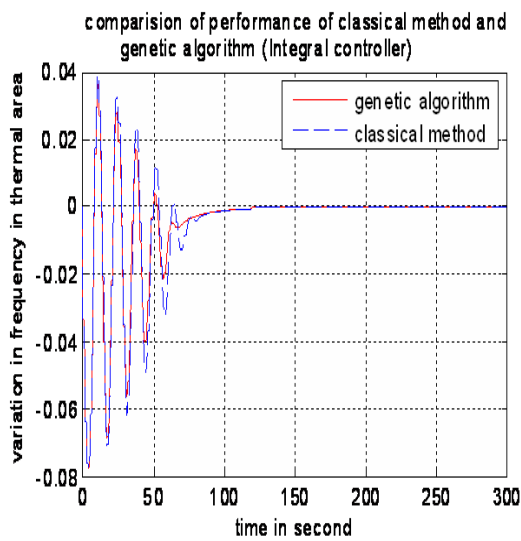
Figure 10. Performance curve between frequency V/s time
