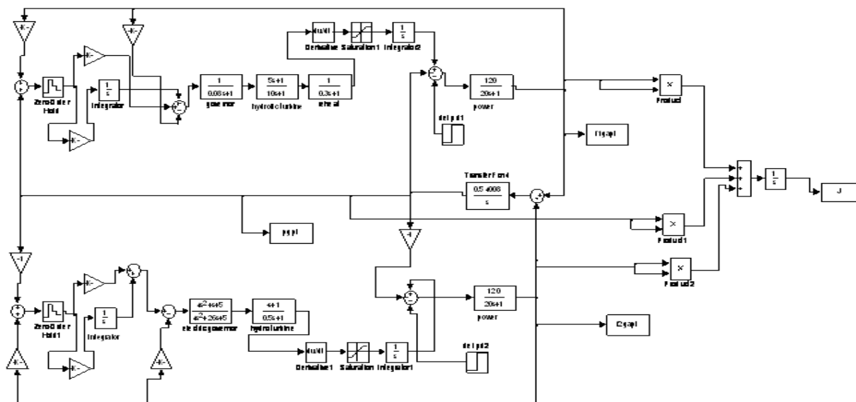
Figure 9. Simulation model of hydrothermal system with GA
