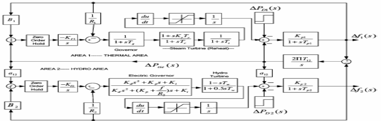
Figure 1. System model for 2 area system
