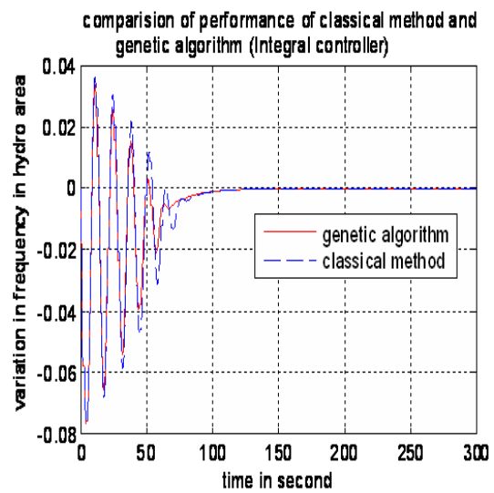
Figure 11. frequency in hydro area v/s time
