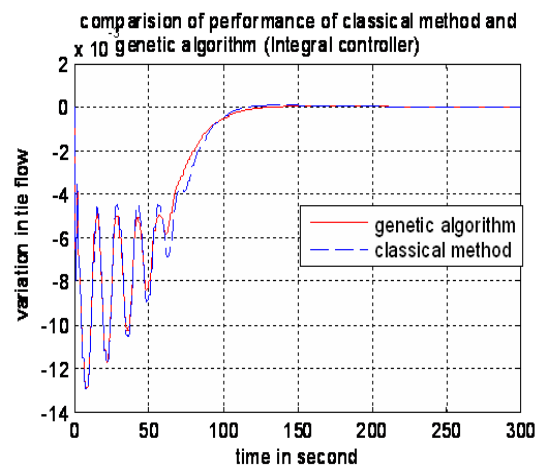
Figure 13. Variation in flow v/s time
