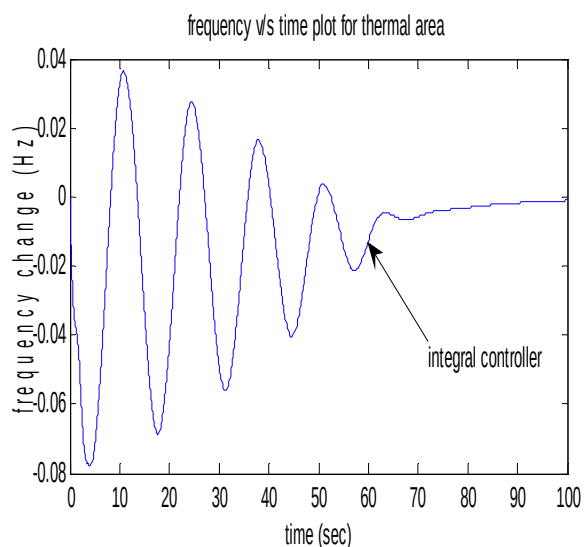
Figure 8. Variation of frequency for 1% step load change in thermal area
